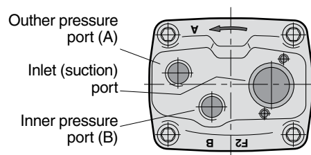
End cap for right hand rotating pump
